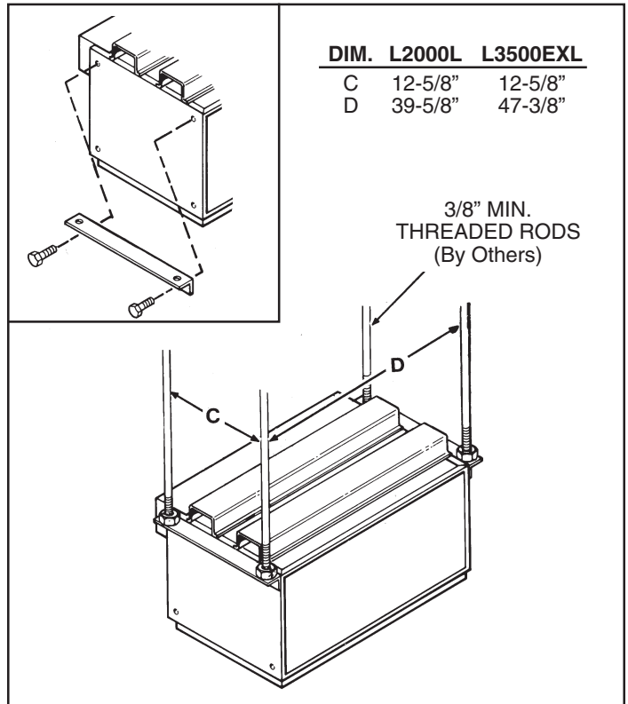
Mounting with threaded rod through adjustable mounting brackets located at top of housing.
