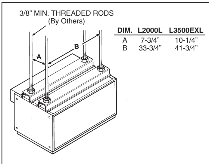
Typical mounting with threaded rod through mounting channels on top of housing.
