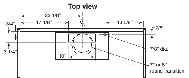
MODEL RMIP45 WITH 331H, 332H, 335, 336, HLB3, HLB6, HLB9 OR HLB11 BLOWER (Vertical Outlet)
