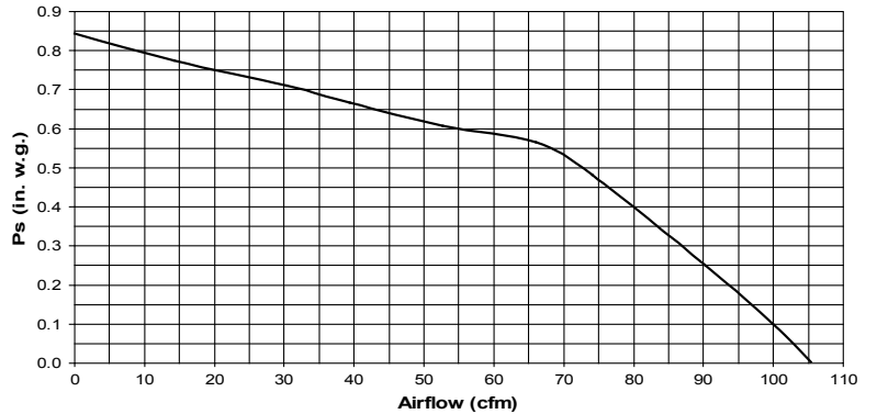
MODEL QTR100FLT
